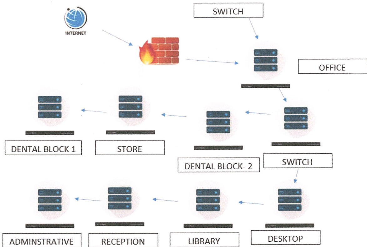
Network Diagram- Server Room to Building Connectivity
